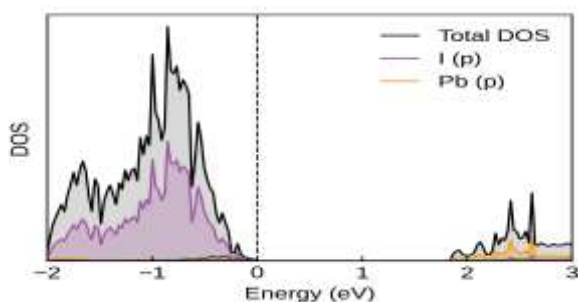
Figure 3.2.1(a) DOS of defective MAPbI 3
