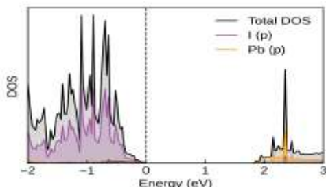
Figure 3.1 (a) Density of States (DOS) of pristine MAPbI 3 Figure 3.1 (b) Band structure of pristine MAPbI 3
