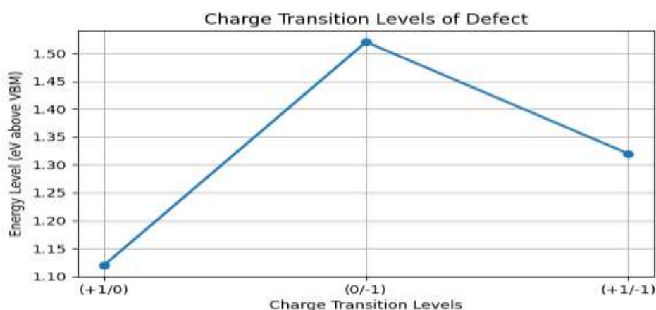
Figure 3.4 Charge transition levels for iodine vacancy
