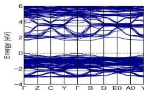
Figure 3.2.1(b) Band of defective MAPbI 3
