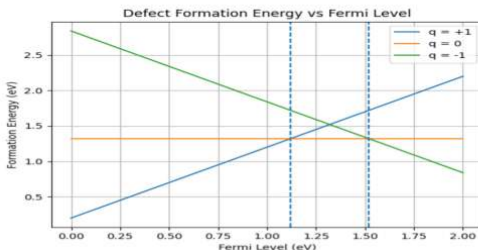
Figure 3.3. Defect formation energy versus Fermi level
