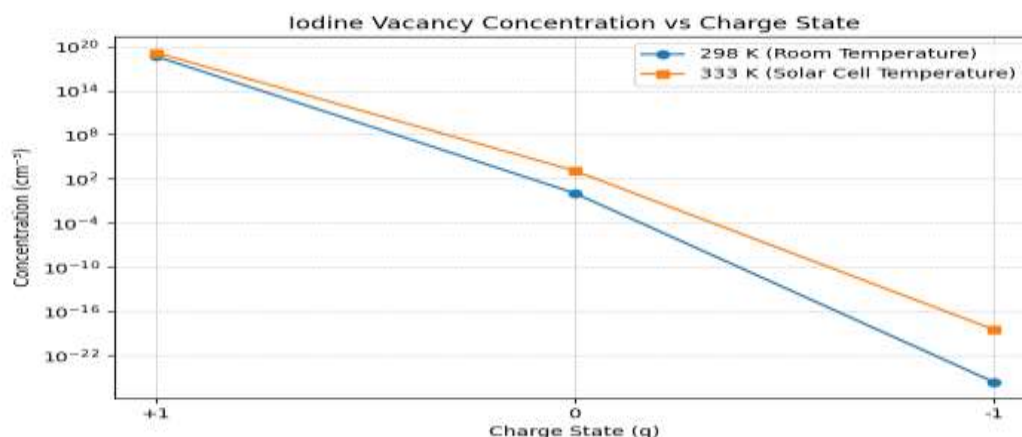
Figure 3.5. Defect concentration plot
